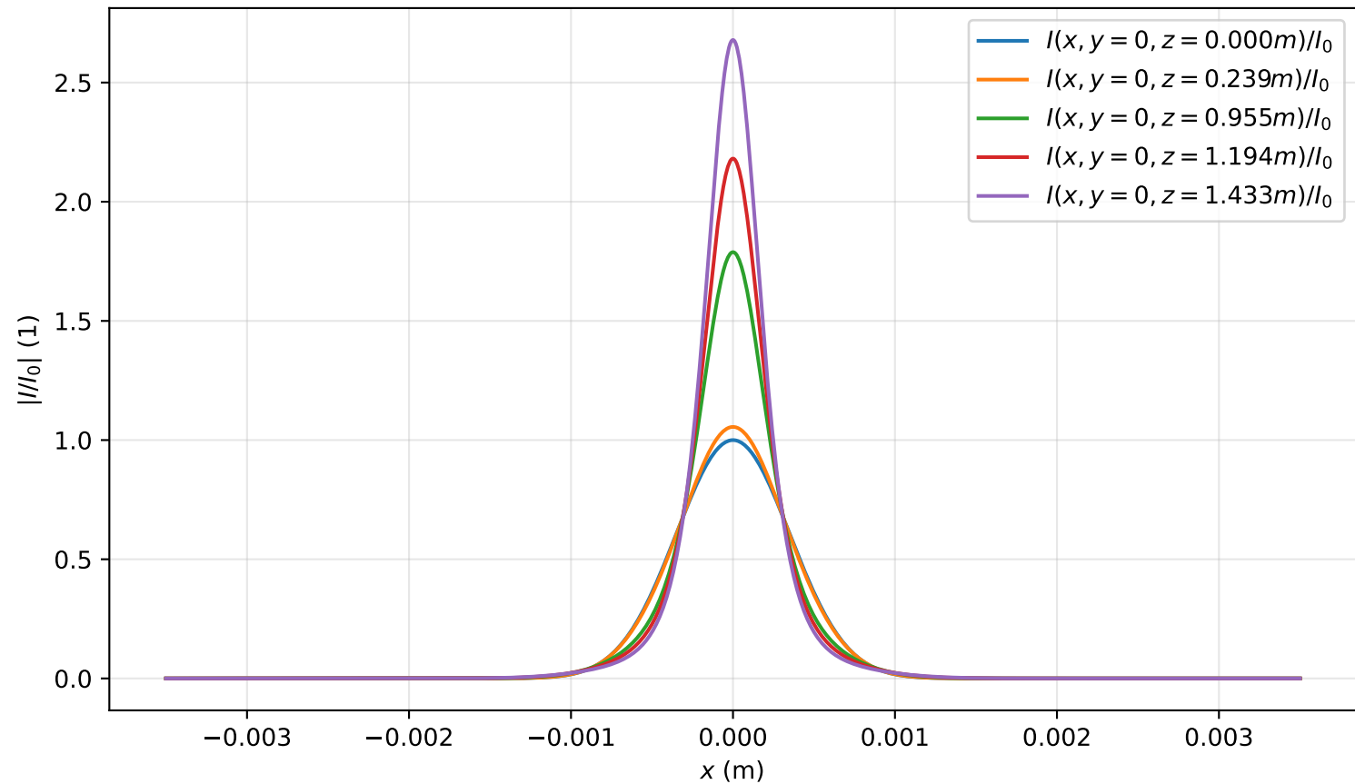
Intensity profile I(x, y = 0, z)/I_0 , P_{in}=1.2P_{cr} , artificial time
